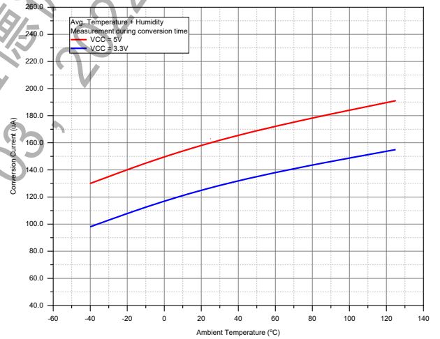
Figure 6. Conversion Current
